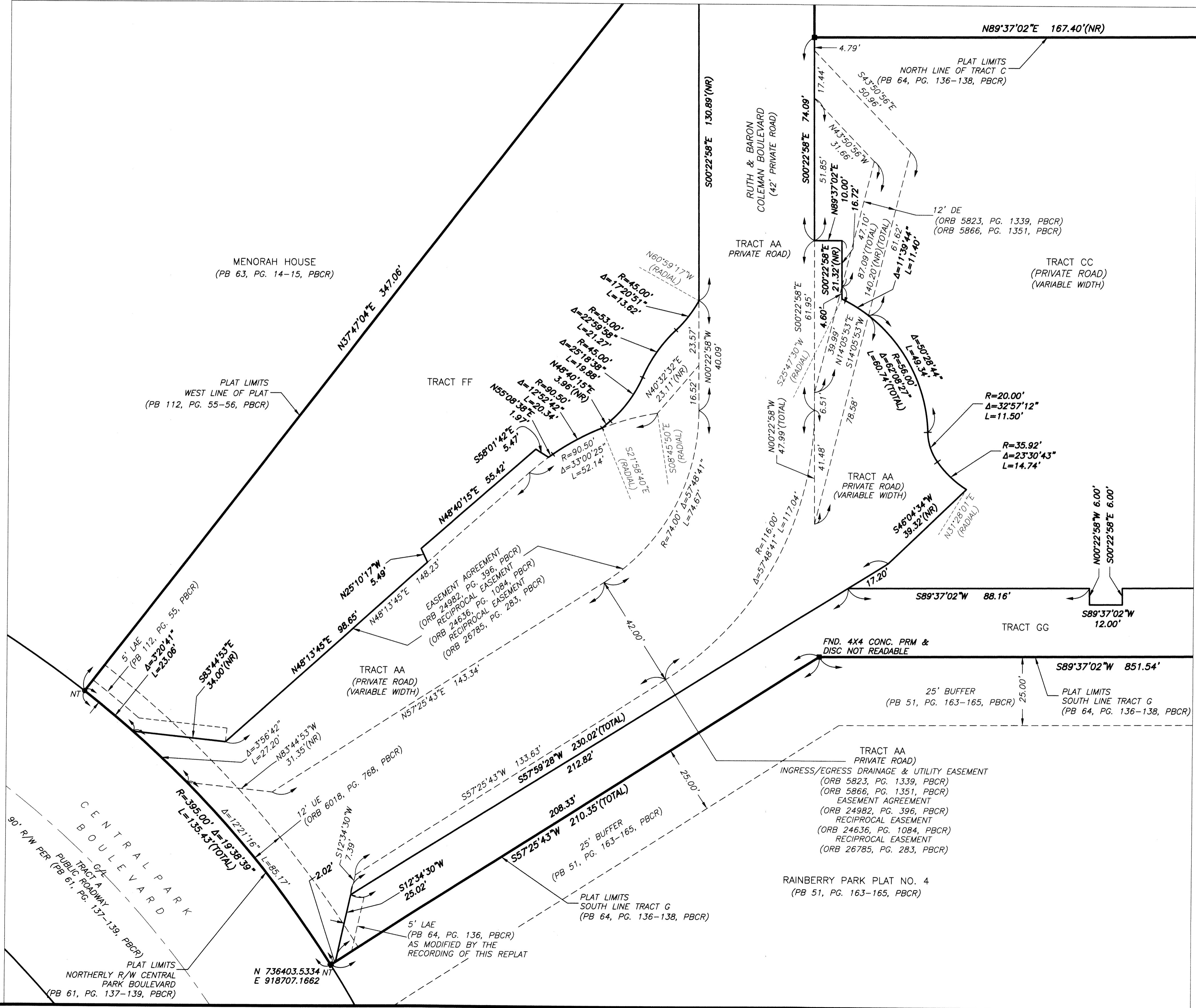
"DETAIL A" FROM SHEET 2
